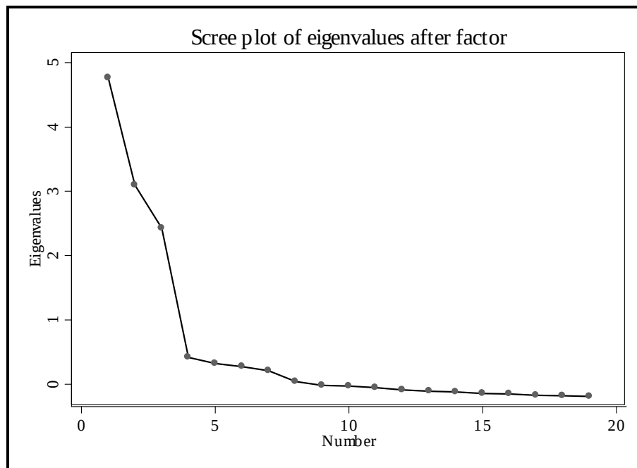
Figure 1: Screeplot for Eigenvalues after the factor analysis of the 19 variables
