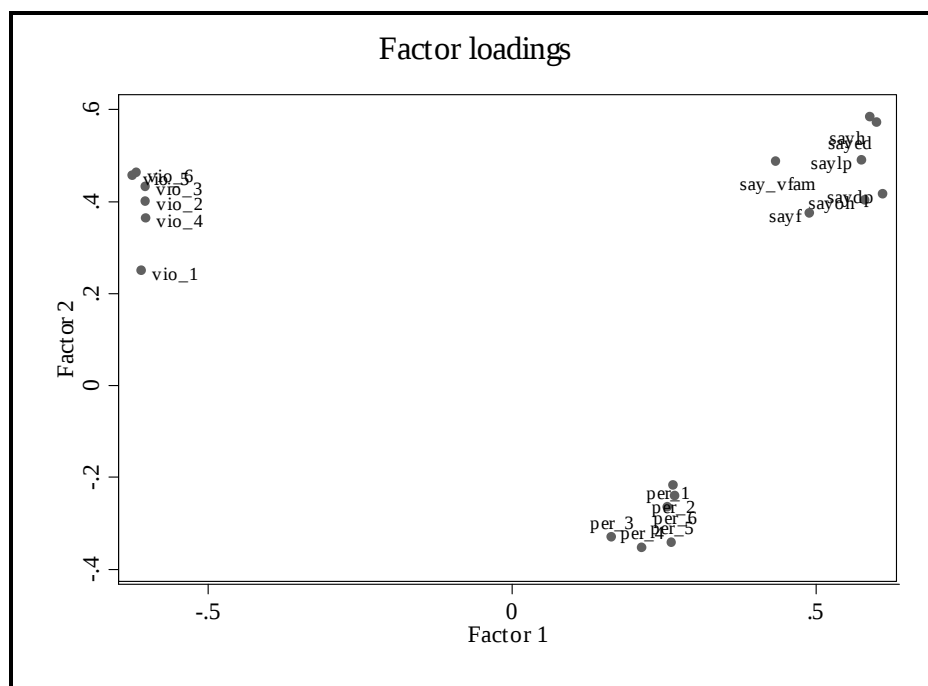
Figure 2: Factor Loadings of the 19 Variables
